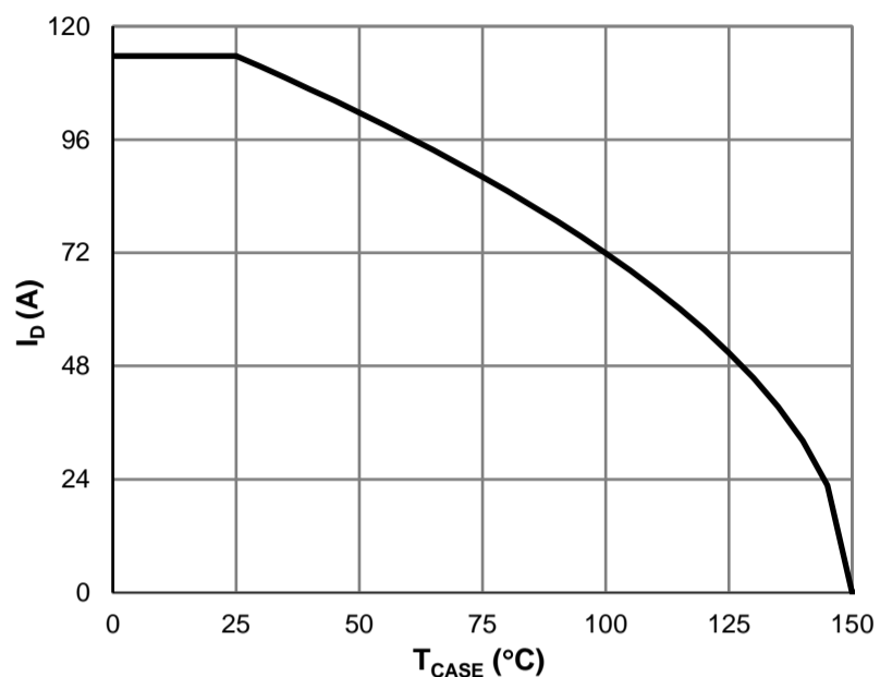
Figure 7: Current De-rating
